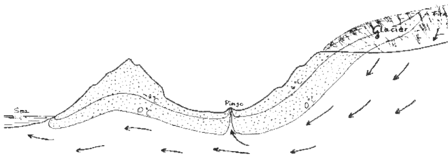
Figure 2. Vertical profile of permafrost zone (dotted) with indication of the -4^{\circ}\text{C} and 0^{\circ}\text{C} isotherm and groundwater movement from a glacier out to the coast. A pingo is shown in the center of the figure.
